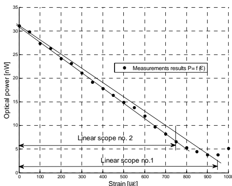
Fig. 9. Chart presenting correlations between the optical power P in the grating strain function after applying the wavelet transformation of measured gratings with a spectrum characteristic.
